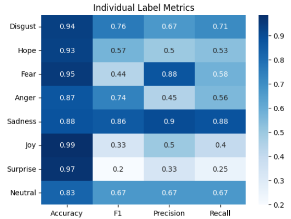
Figure 3: Individual label accuracy, precision, recall and F-1 score of our system on the development dataset.
