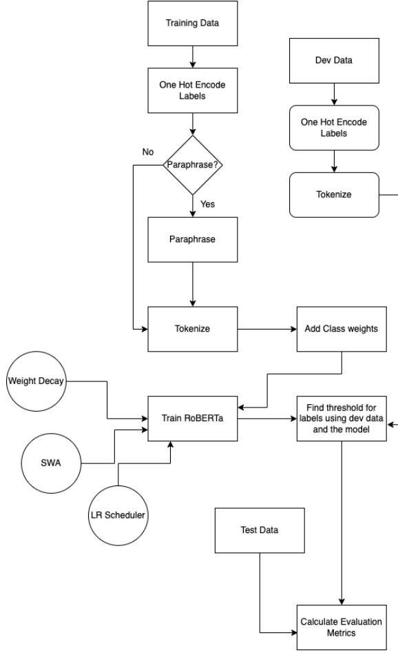
Figure 2: High-level flowchart of our proposed system.
